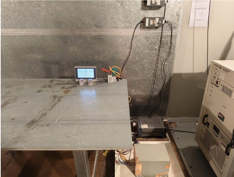
Photograph 2: Set-up for conducted emission, Ethernet ports
