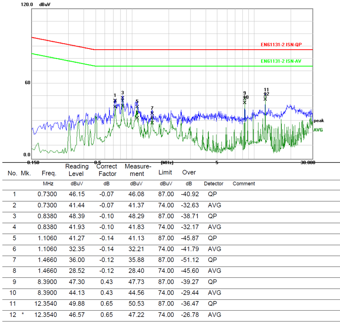
Figure 4: Spectral Diagrams, Conducted emission, 0.15-30MHz, LAN, RJ45-2
