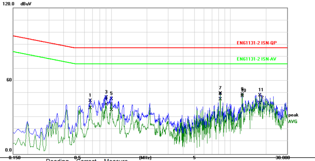
Figure 3: Spectral Diagrams, Conducted emission, 0.15-30MHz, LAN, RJ45-1
