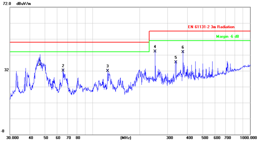
Figure 7: Spectral Diagrams, Radiated Emission, 30MHz-1GHz, Vertical
